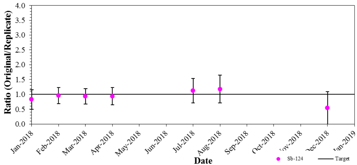
Image 7.10: Performance du Sb-124 (AQ interne – Double/multiple)
