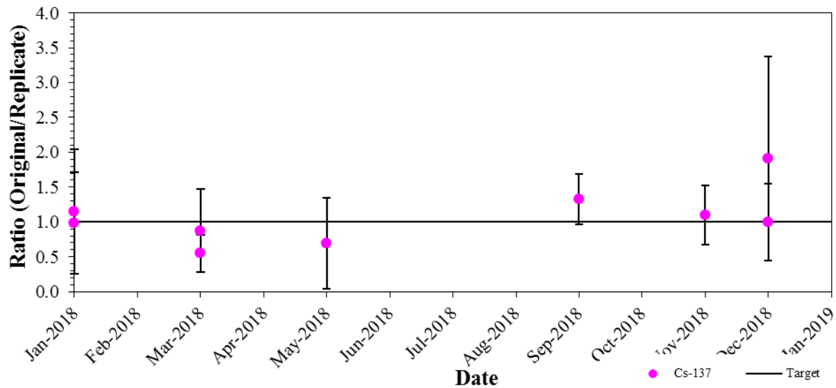
Image 7.06: Performance du césium-137 (AQ interne – Double/multiple)
