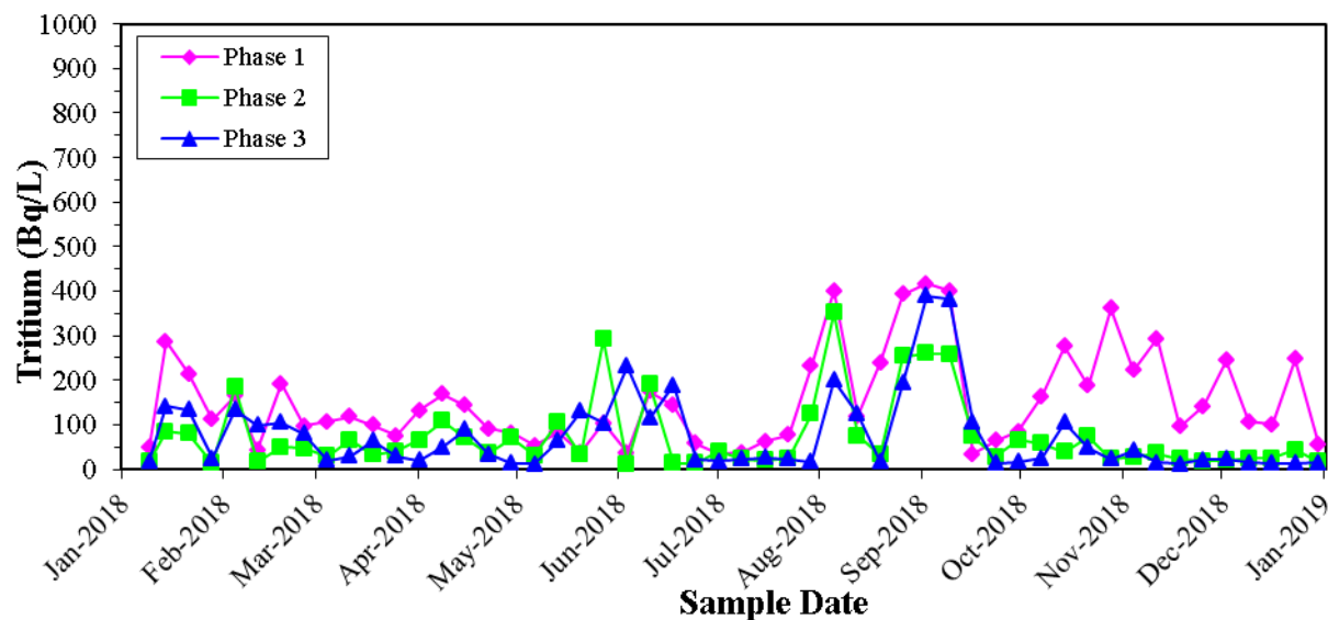
Image 4.22: Tritium (eau du canal Parshall, IGDRS)
